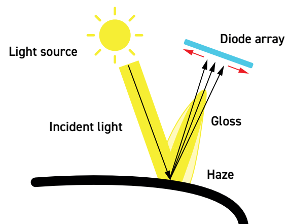
The IQ Flex 20-S automatically adjusts for non-flat surfaces by sensing the reflected peak and virtually adjusting the position of the sensor.
