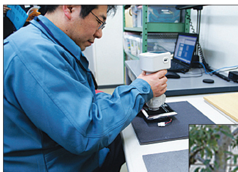
Bluetooth transfers measured color data to PC
